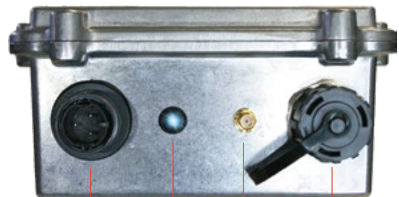
power supply status LED GSM/GPRS antenna Ethernet
